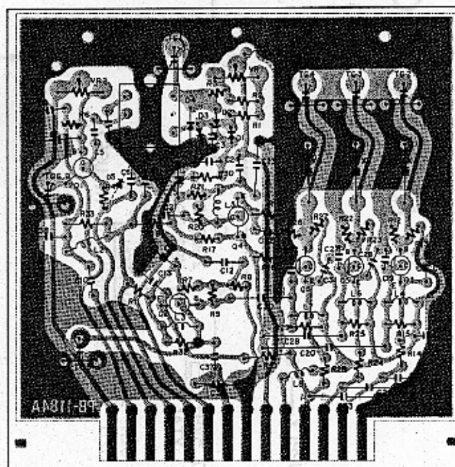
Viewed From Solder Side
