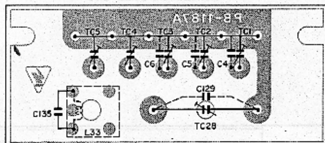
Viewed From Component Side
