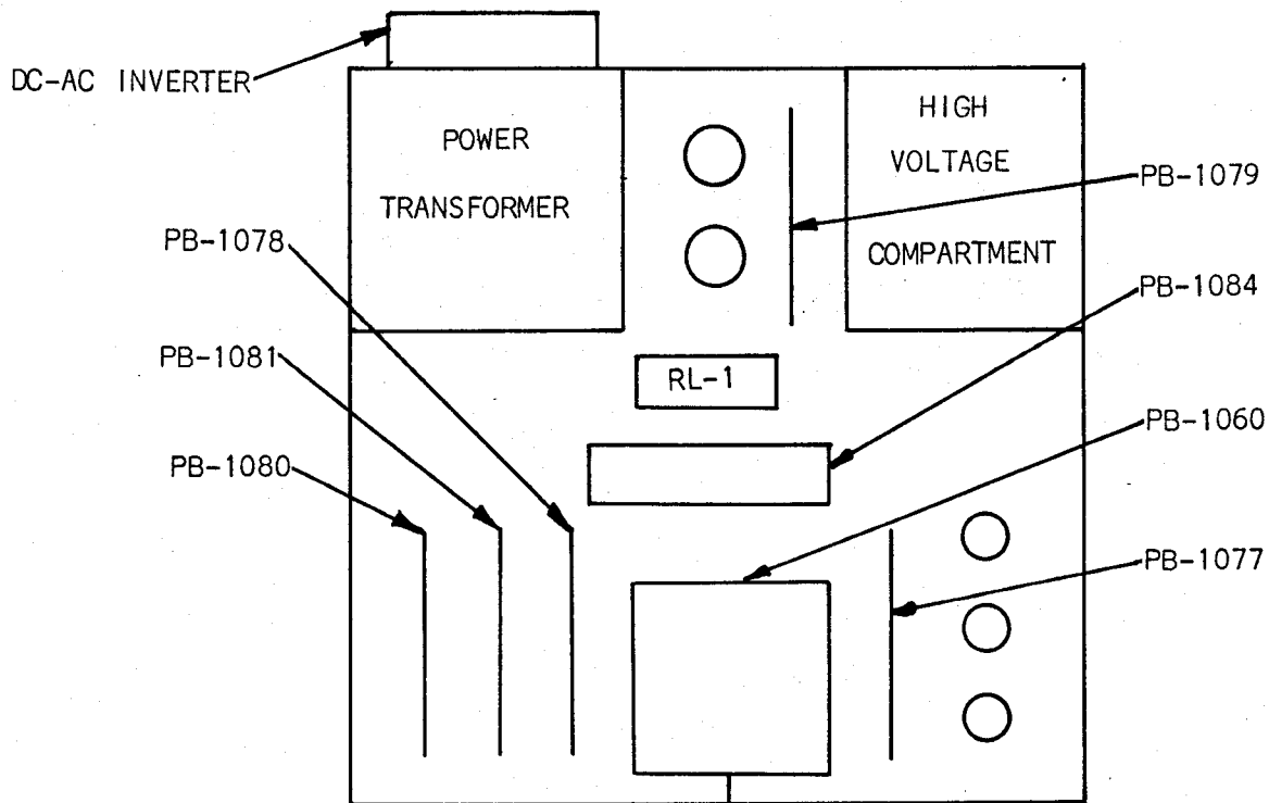
FT-101 EARLY Serial No. 025000 & down
